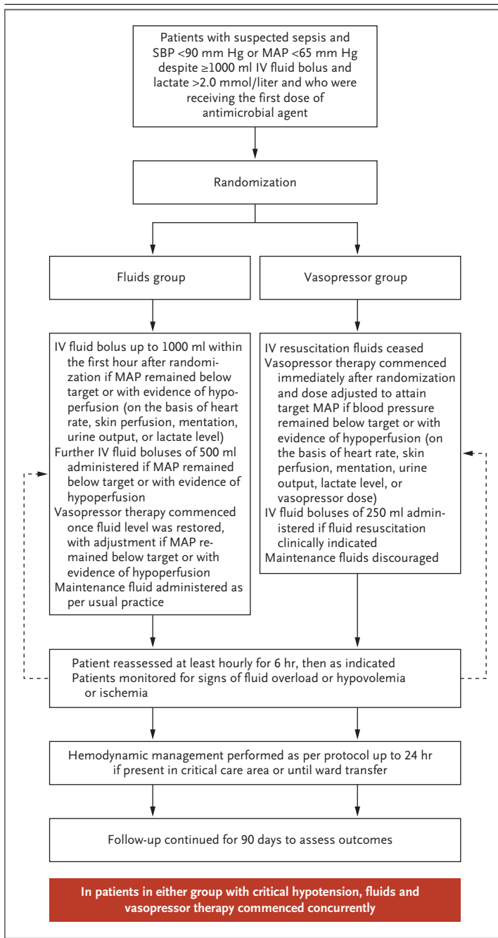
Figure 1. Trial Algorithm.
